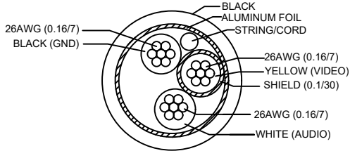
SECTION A-A CABLE BUILDUP
