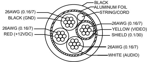
SECTION B-B CABLE BUILDUP
